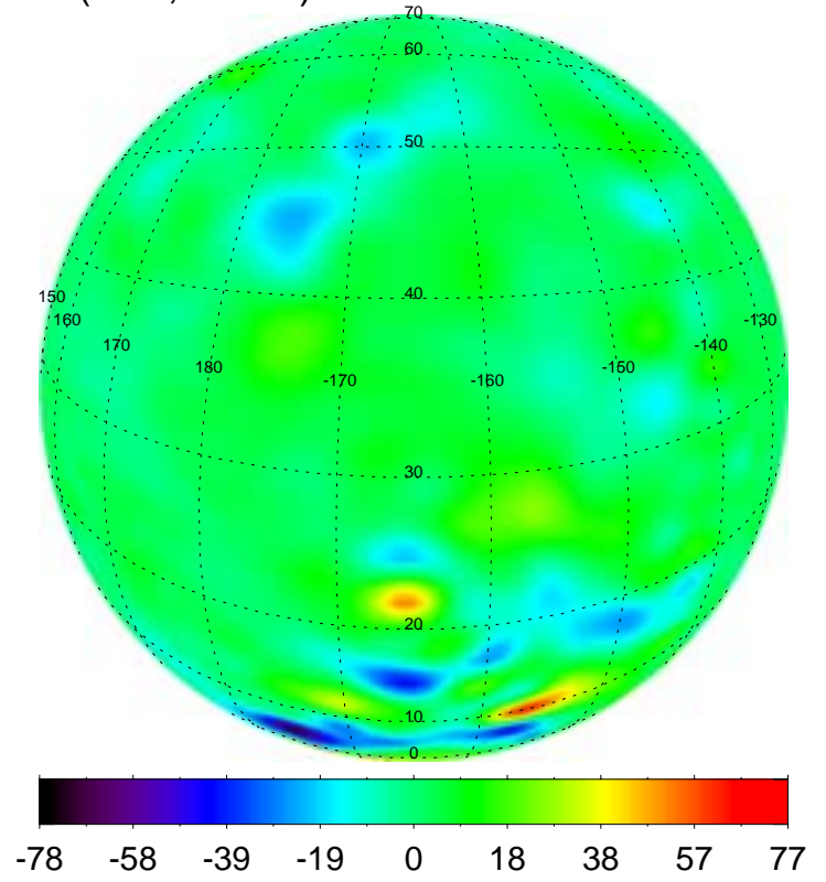
X (35N, 165W) Amizonis Planitia 200 km
