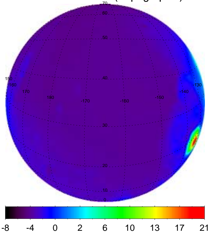
Amizonis Planitia (Topographic)
