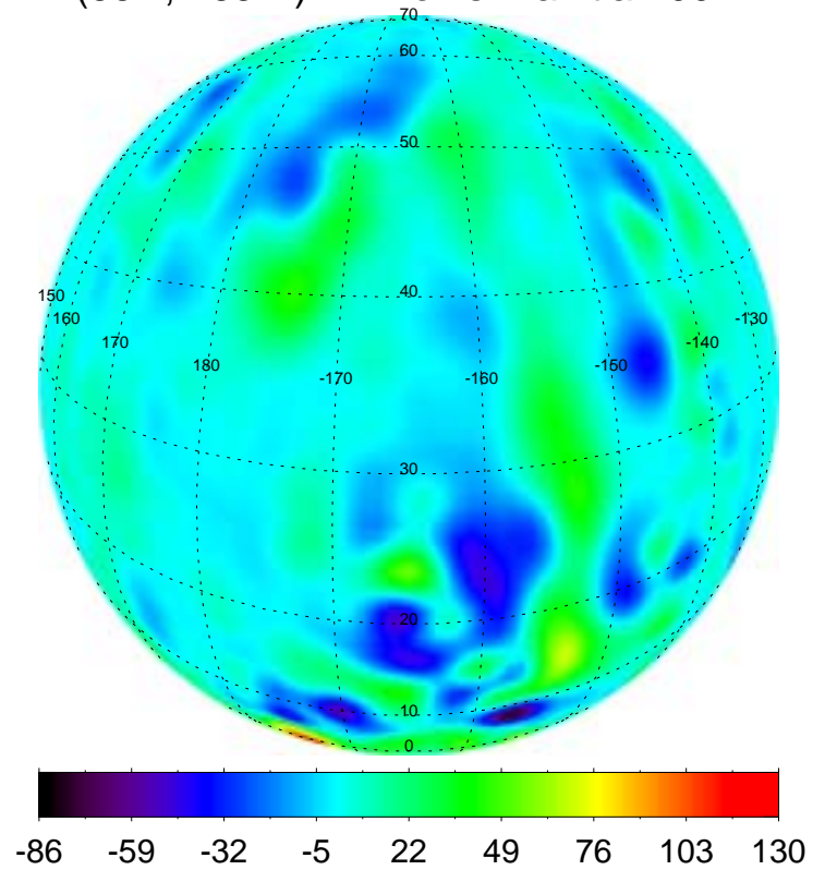
Z (35N, 165W) Amizonis Planitia 200 km
