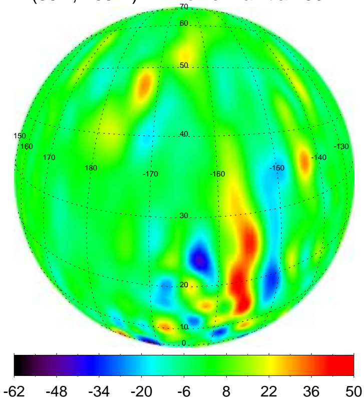
Y (35N, 165W) Amizonis Planitia 200 km
