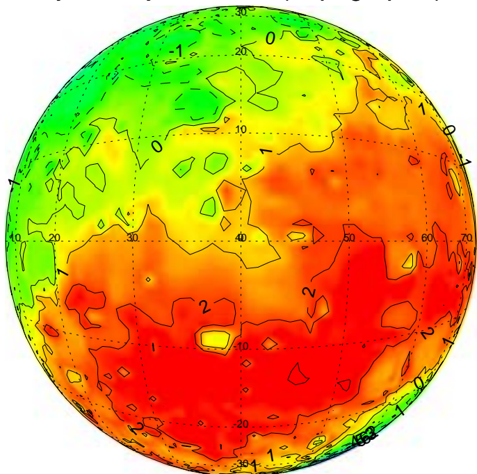
Syrtis Major Planum (Topographic)
